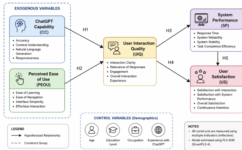
Figure 1. Research Framework Diagram Evaluating the Effectiveness of ChatGPT in Web-Based Information Systems
